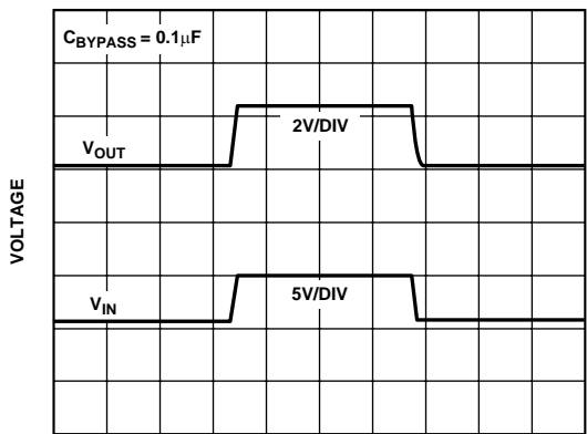
Figure 34. ADR391 Turn-Off Response at 15 V
