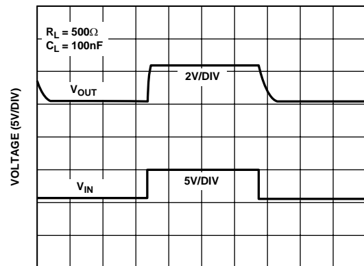
Figure 36. ADR391 Turn-On/Turn-Off Response at 5 V
